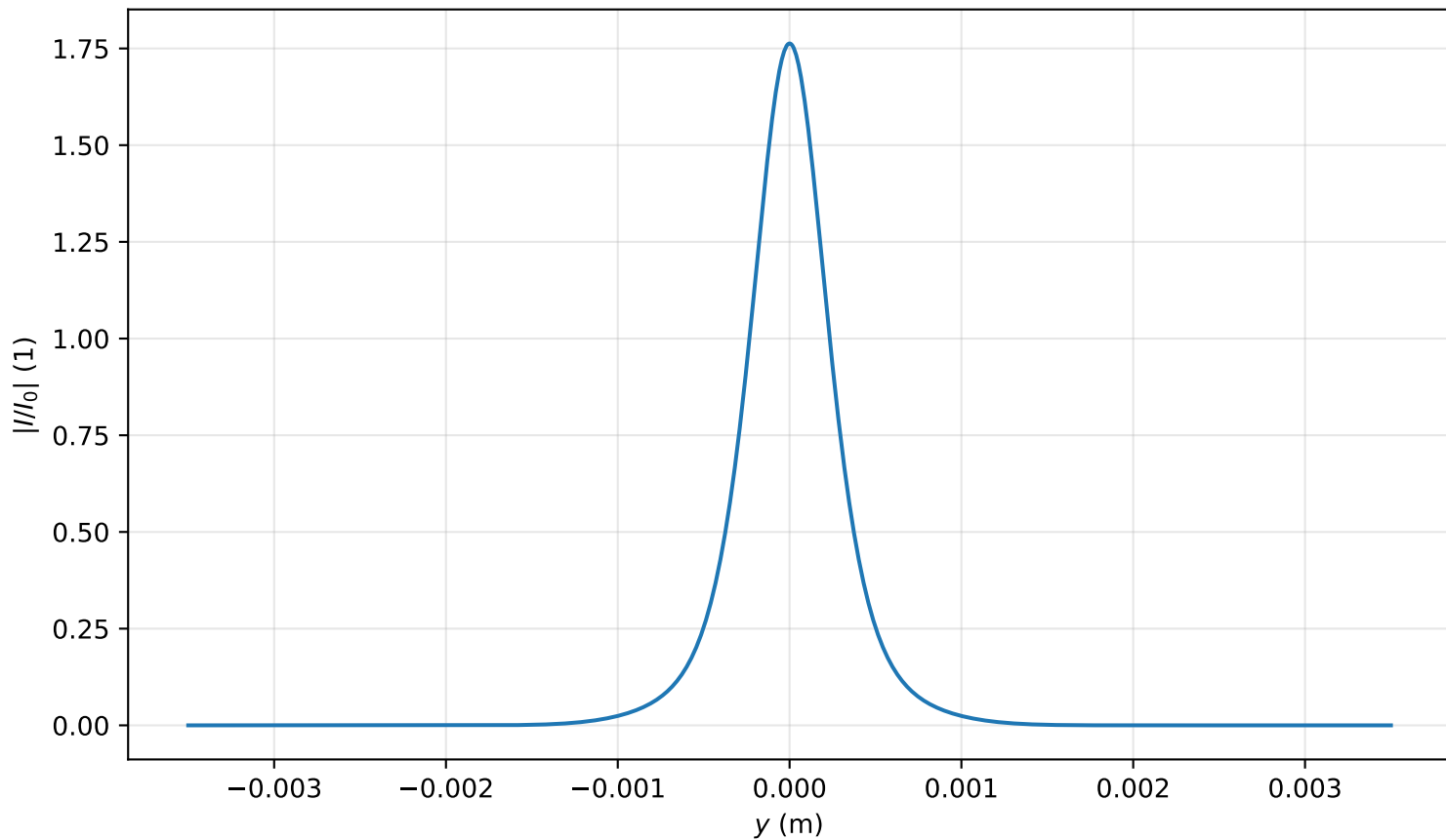
Intensity profile I(x=0, y, z=1.353)/I_0 , P_{in}=1.0P_{cr} , artificial time
